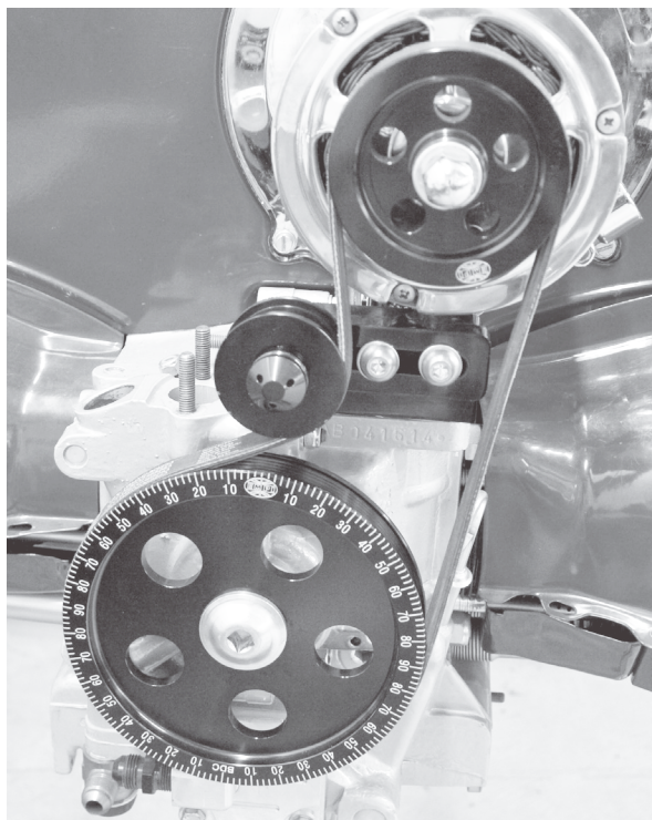
8. Install the Serpentine Alternator pulley. Be sure to face the raised hub outward.
