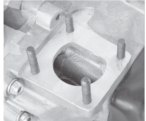
4. Install the new Studs furnished in the kit. Thread them down completely into the case.
