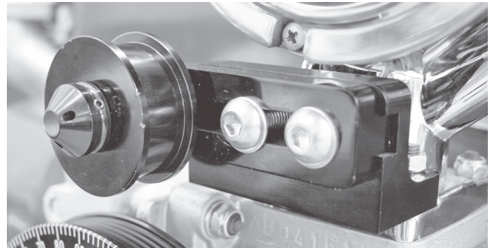
5. Re-install the Alternator stand and the new Idler Bracket. The ears of the bracket face down, with the Pulley facing to the left hand side of the motor.
